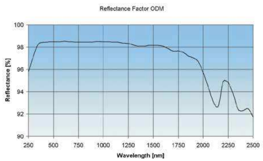
WS-2 curve
