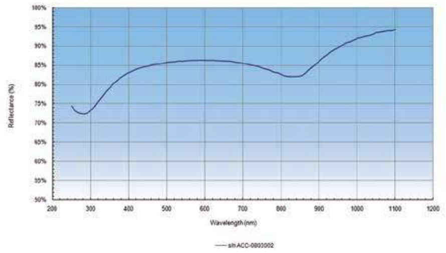
RS-2 curve
